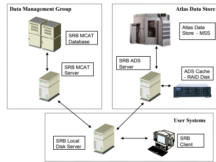
CCLRC Data Archival Management Architecture
